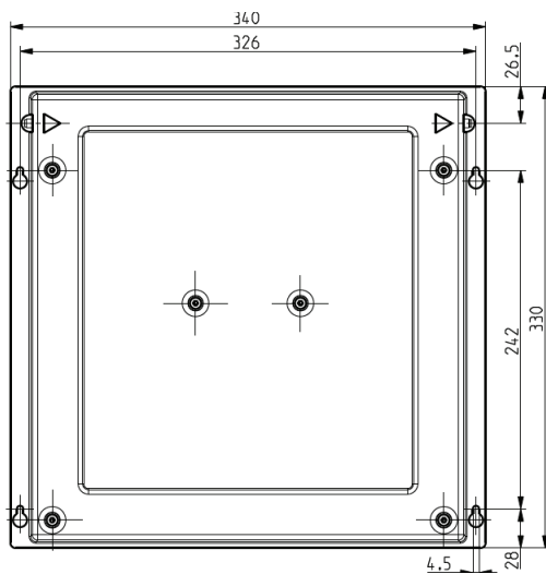
Front view with Smart Shelf antenna
